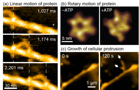
Fig. 1: Nanoscale life phenomena visualized by high-speed AFM. (a) Myosin V walking along the actin filament. (b) Rotary catalysis of rotor-less F1-ATPase. (c) Filopodia growth from living nerve cell.
