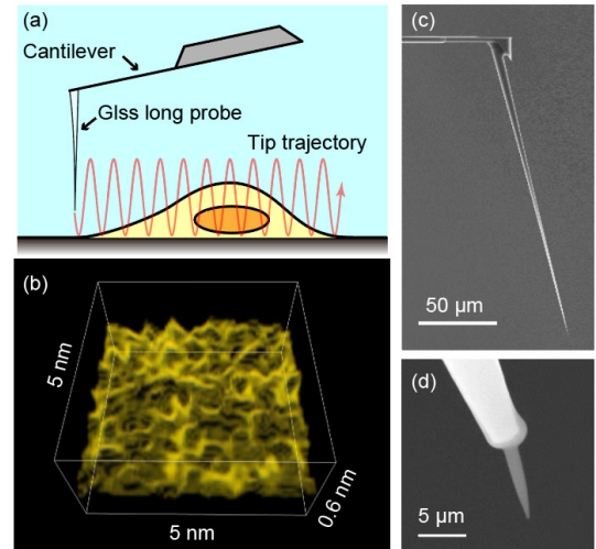
Fig. 4: (a) Nano-endoscopic imaging of inside a cell. (b) 3D-AFM image of molecular adsorption structures obtained at a solid/liquid interface. (c) Glass probe attached to an AFM cantilever. (d) EBD tip fabricated on a glass probe.
