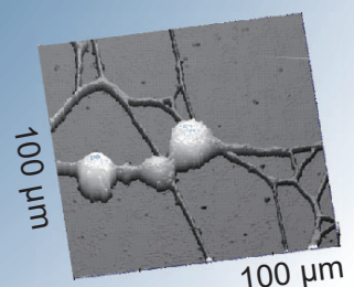
SICM Y. Takahashi et al. Angew. Chem. Int. Ed. 2011.
