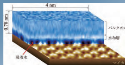
Water distribution on Mica T. Fukuma et al. Phys. Rev. Lett. 2010.
